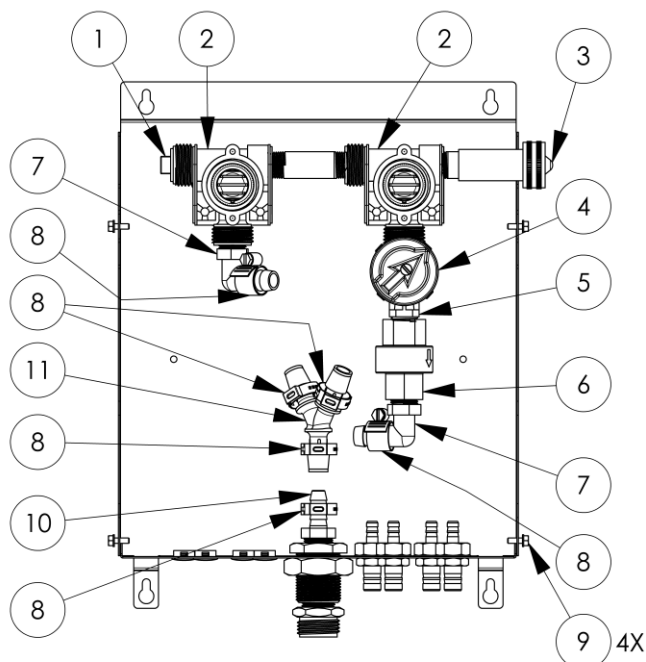
FRONT VIEW : NO COVER HARDWARE & VALVES
